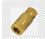
MC 20F2:1/4" Female MC 30F2:3/8" Female Material: Brass/Steel/Zinc
