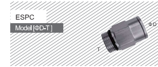
Tube(Metric)-Thread(PT): ESPC 4-G01 ESPC 4-G02 ESPC 6-G01 ESPC 6-G02 ESPC 6-G03 ESPC 8-G01 ESPC 8-G02 ESPC 8-G03 ESPC 8-G04 ESPC 10-G02 ESPC 10-G03 ESPC 10-G04 ESPC 12-G02 ESPC 12-G03 ESPC 12-G04 ESPC 4-M5 ESPC 4-M6 ESPC 6-M5 ESPC 6-M6
